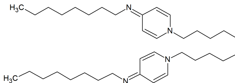
Figure 1. Chemical structure of octenidine.
